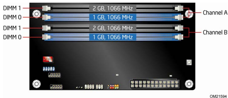
Figure 19. Example Dual Channel Memory Configuration with Four DIMMs
