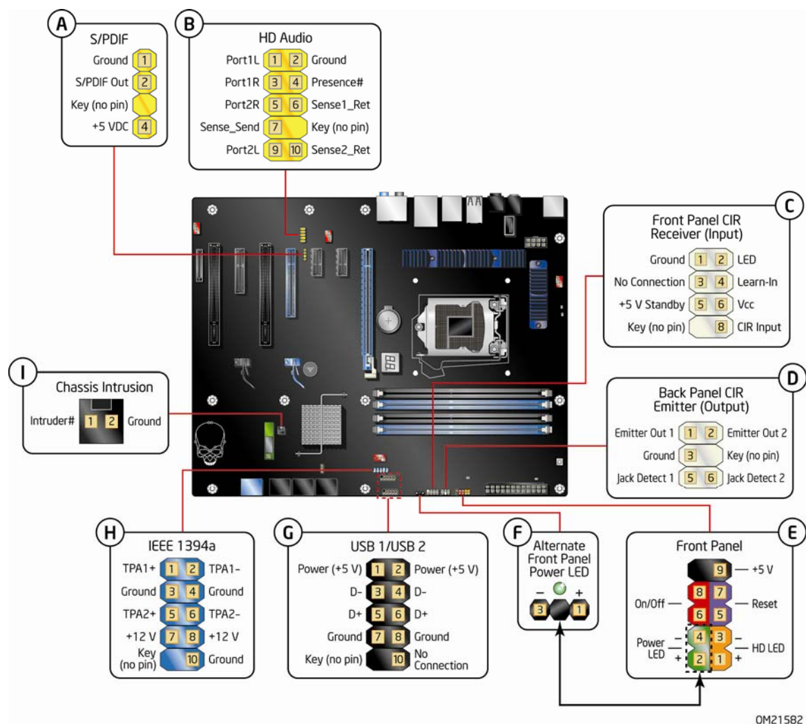
Figure 27. Internal Headers
