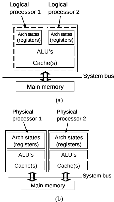
Figure 1: High-level diagram of (a) a processor with Hyper-Threading Technology and (b) a dual-processor system
